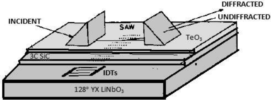
Figure 1: TeO 3 ( )/3C-SiC()/128°Y-X LiNbO 3 multilayered acousto optic device configuration with IDTs placed on the top of LiNbO 3 crystal.
